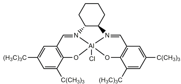
(S, S)-Jacobsen's Salen Al catalyst
